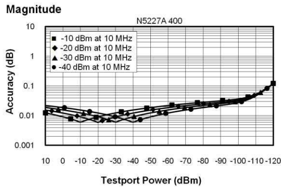
N5227A Dynamic Accuracy, 10 MHz - Specification
