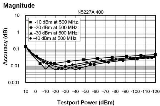
N5227A Dynamic Accuracy, 500 MHz - Specification
